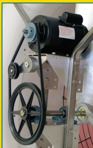
Motor mount and drive assembly utilize a rugged box frame design to increase motor life.
